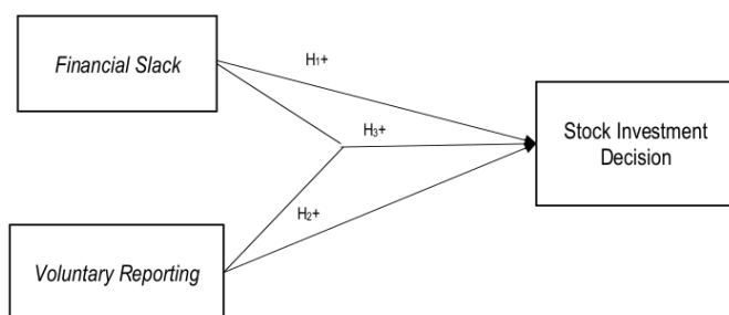
Figure 1. Research Model
