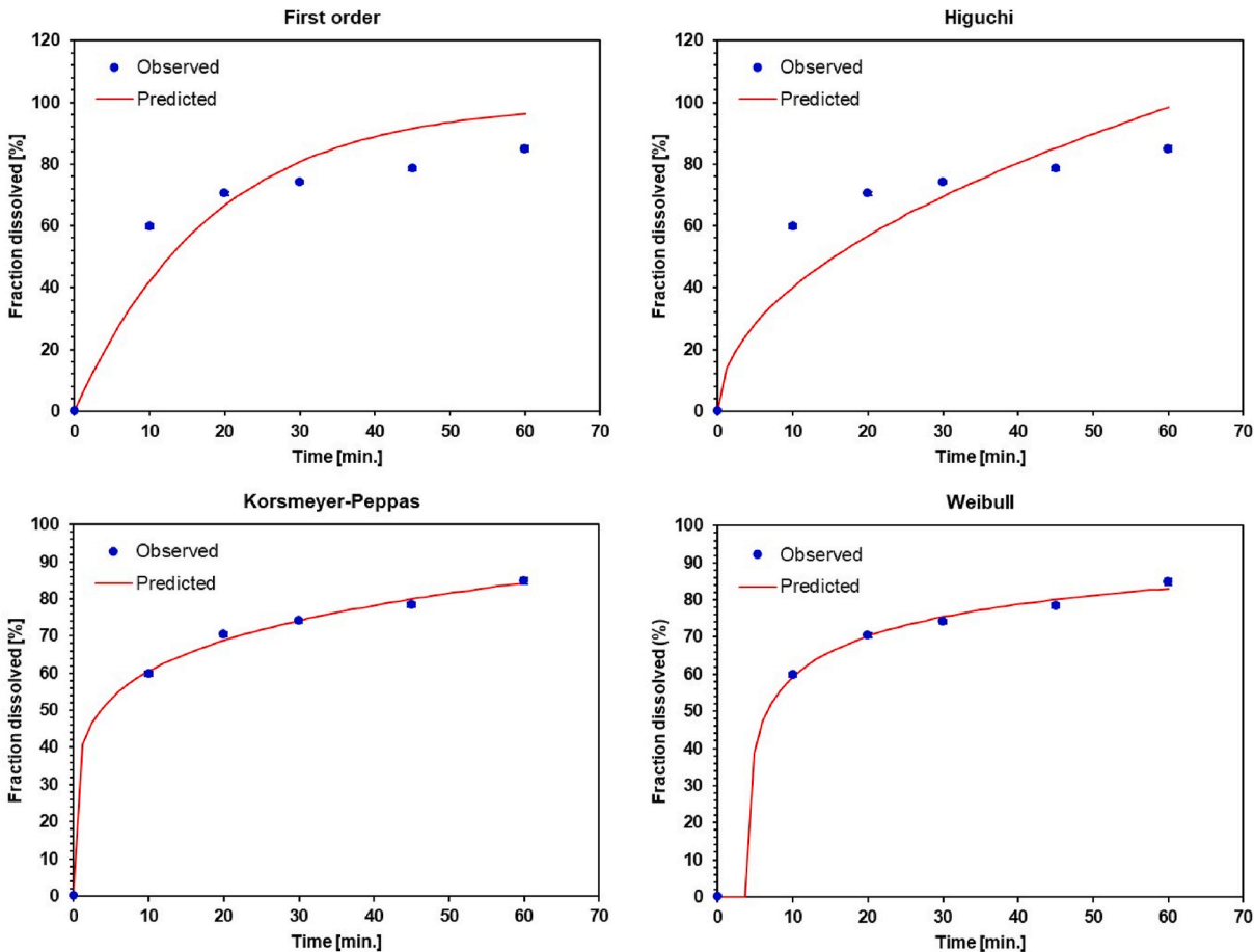
Fig. 7. Release kinetics model of 4CH 2 Cl from Ta, Tb, Tc, and To tablets. The compositions of SSG [mg] and PVP K-30 [mg] are Ta (40.00 : 16.00) (Korsmeyer-Peppas), Tb (32.00 : 24.00) (Weibull), Tc (24.00 : 32.00) (First order, and To (33.60 : 22.40) (Weibull).
