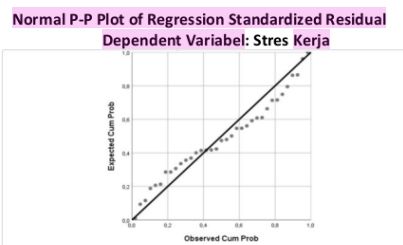
Gambar 2. Hasil Pengujian Probability Plot
