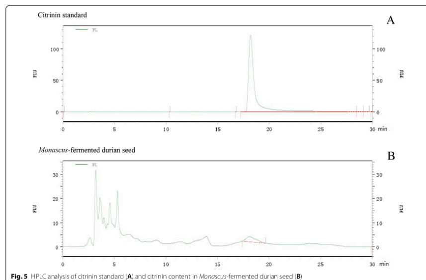
Fig. 5 HPLC analysis of citrinin standard (A) and citrinin content in Monascus -fermented durian seed (B)
