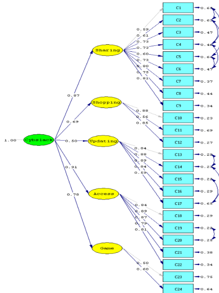
Gambar 1. Second Order CFA Adopsi Skala Cyberslacking
