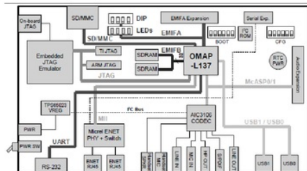
Gambar 2a. Diagram blok Texas Instruments OMAP-L137.
