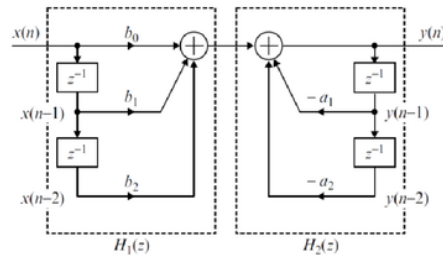
Gambar 1. Diagram blok Direct Form I Structure
