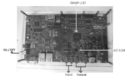
Gambar 2b. Gambar fotograf Texas Instruments OMAP-L137.
