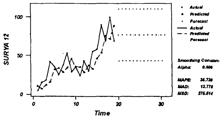
Single Exponential Smoothing
