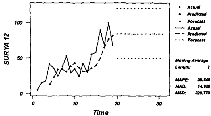
Moving Average
