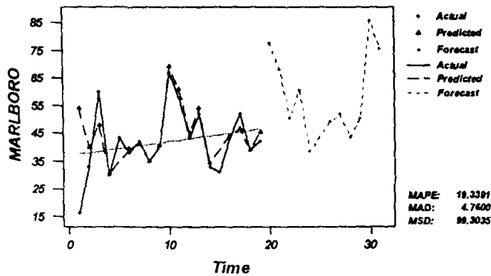
Decomposition Fit for MARLBORO
