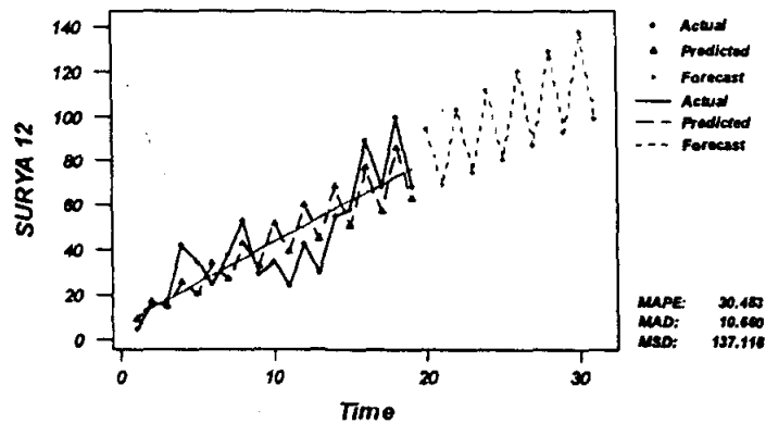
Decomposition Fit for SURYA 12
