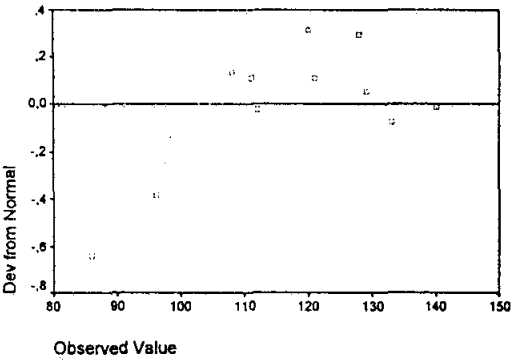
Detrended Normal Q-Q Plot of MANDIRI
