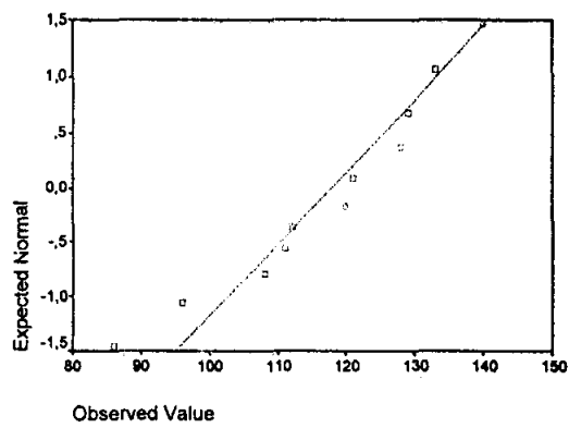
Normal Q-Q Plot of MANDIRI
