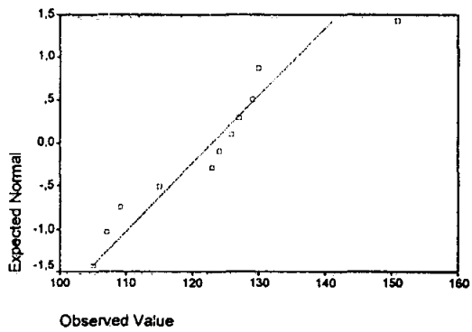
Normal Q-Q Plot of MANDIRI
