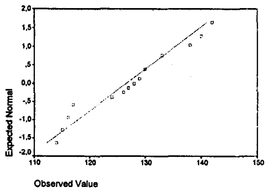
Normal Q-Q Plot of MANDIRI
