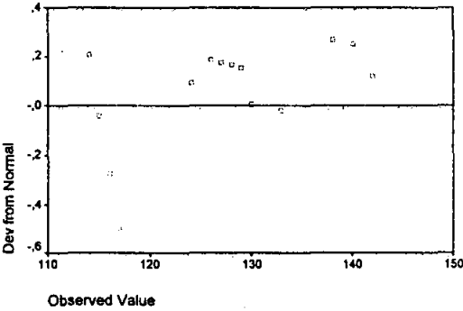
Detrended Normal Q-Q Plot of MANDIRI
