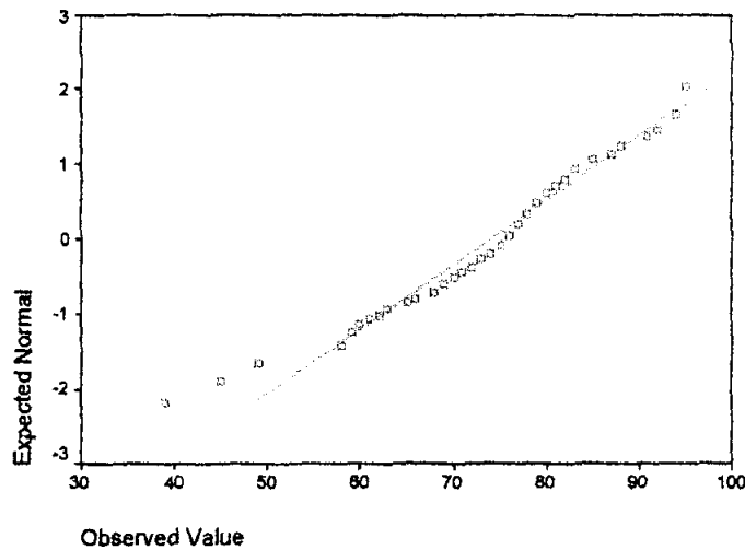
Normal Q-Q Plot of RELASI
