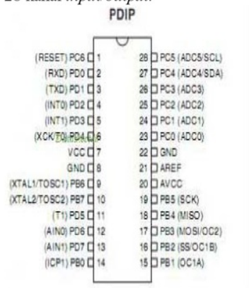
Gambar 1. Pin Out ATmega8L
