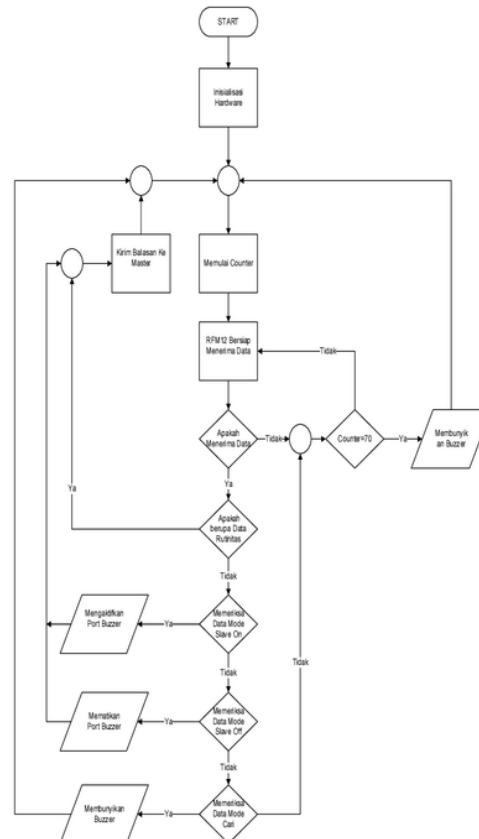
Gambar 14 Flowchart Program Slave
