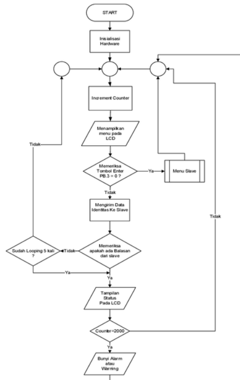
Gambar 12 Flowchart Program Master
