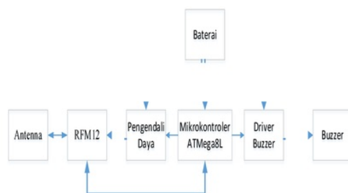
Gambar 4. diagram blok master
