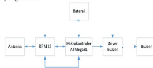
Gambar 5. Diagram Blok Slave
