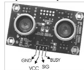
Gambar 1. DT-Sense UltraSonic and InfraRed Ranger
