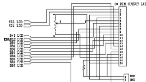
Gambar 9. Rangkaian Driver LCD
