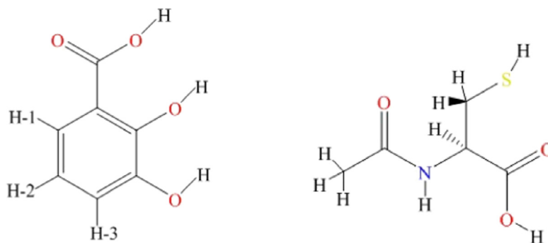
Fig. 3. Structure of ligand Dhba (left) and Nac (right).
