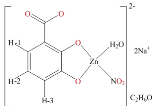
Fig. 4. Proposed structure of zinc binary complex.
