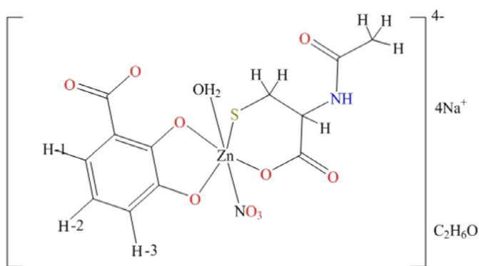
Fig. 5. Proposed structure of zinc ternary complex.
