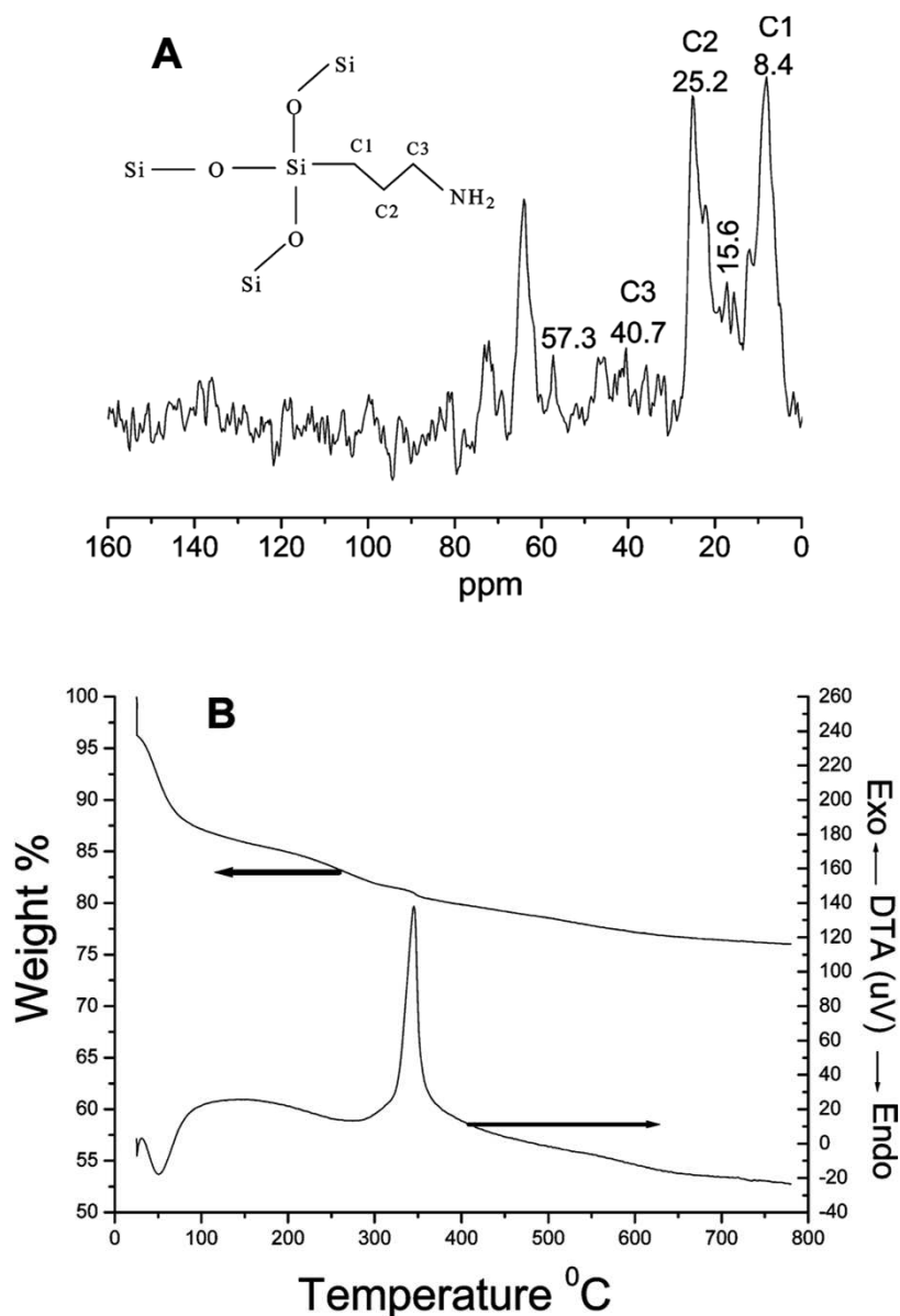
Figure 8. (A) ^{13}\text{C} NMR spectra (B) TGA analysis of the sample APTES 15-160-1/15.
