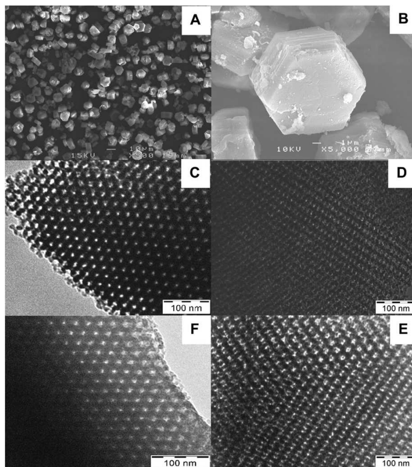
Figure 3. SEM images (A,B) and TEM images (C,D) of APTES 15-160-1/15, and TEM images of PS (E,F).
