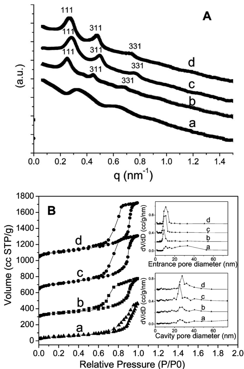
Figure 6. SAXS spectra (A) and \text{N}_2 sorption isotherms (B) of amine FDU-12 samples synthesized with different amount of APTES: (a) APTES 15-160-1/7.5, (b) APTES 15-160-1/10, (c) APTES 15-160-1/15, and (d) APTES 15-160-1/20. (inset in B: cavity pore size or entrance pore size distribution). The isotherm curves b, c, and d are shifted by 300, 600, and 1000 cc \text{g}^{-1} STP, respectively, for clarity.
