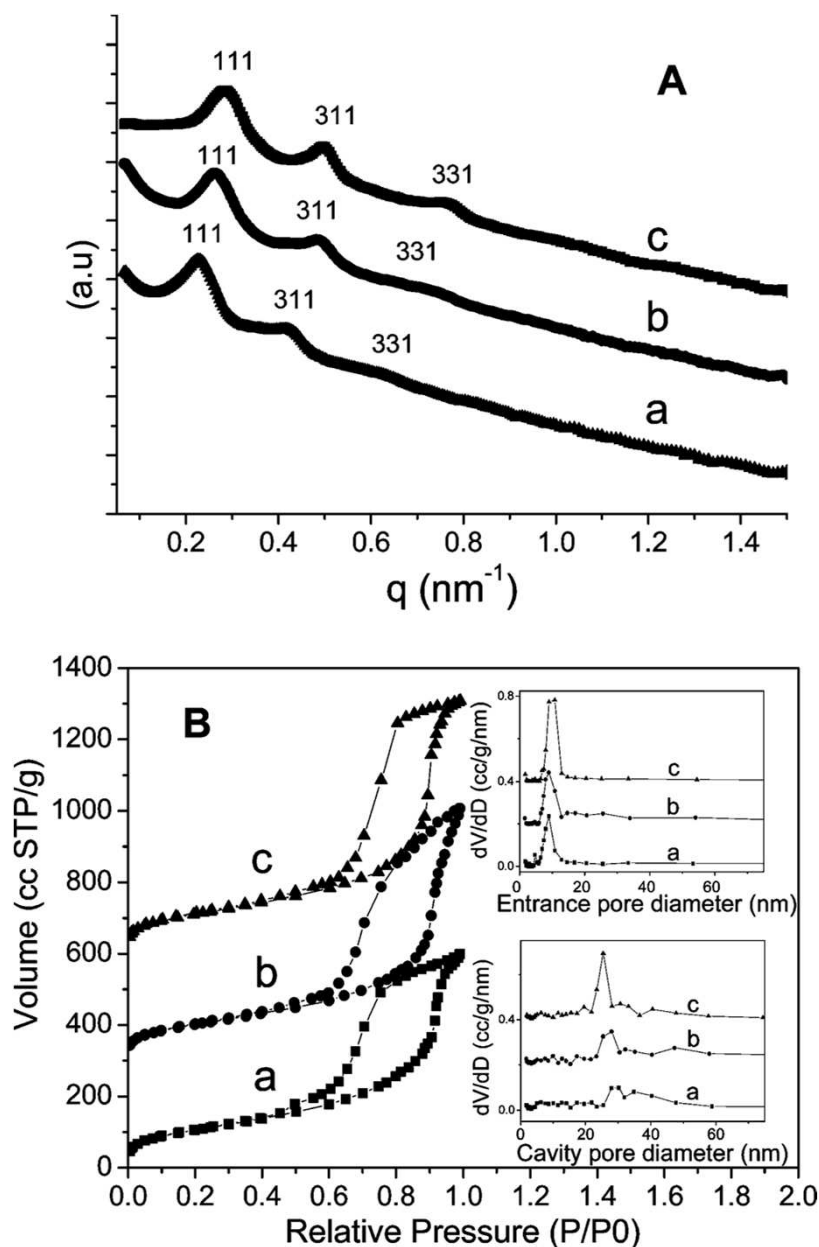
Figure 4. SAXS spectra (A) and N_2 sorption isotherms (B) of amine FDU-12 samples synthesized at different reaction temperatures: (a) APTES 10-160-1/15, (b) APTES 12-160-1/15, and (c) APTES 15-160-1/15. (inset in B: cavity pore size distribution or entrance pore size distribution). The isotherm curves b and c are shifted by 300 and 600 \text{cc g}^{-1} STP, respectively, for clarity.
