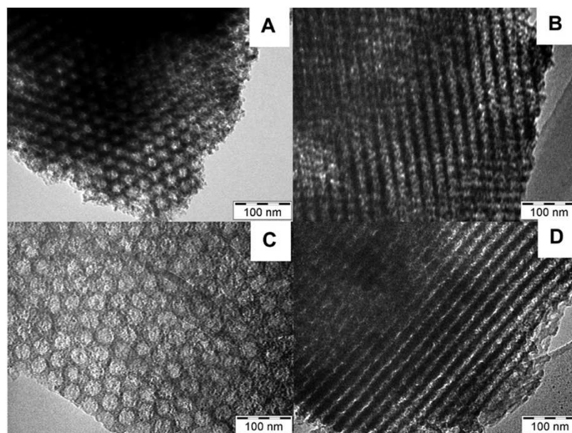
Figure 5. TEM images of amine FDU-12 samples synthesized at different reaction temperatures: APTES 12-160-1/15 (A,B) and APTES 10-160-1/15 (C,D).
