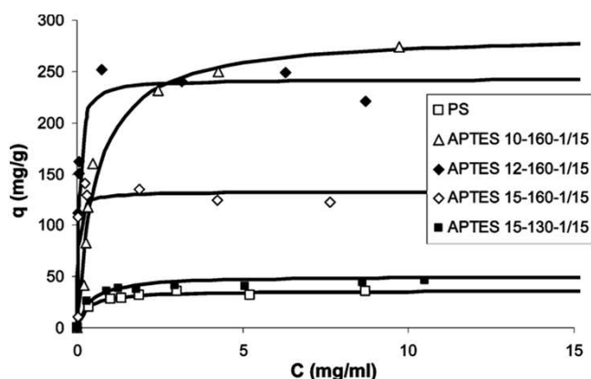
Figure 9. Adsorption isotherms of BSA on FDU-12 PS and amine FDU-12 samples with different cavity and entrance sizes (at 20 °C).
