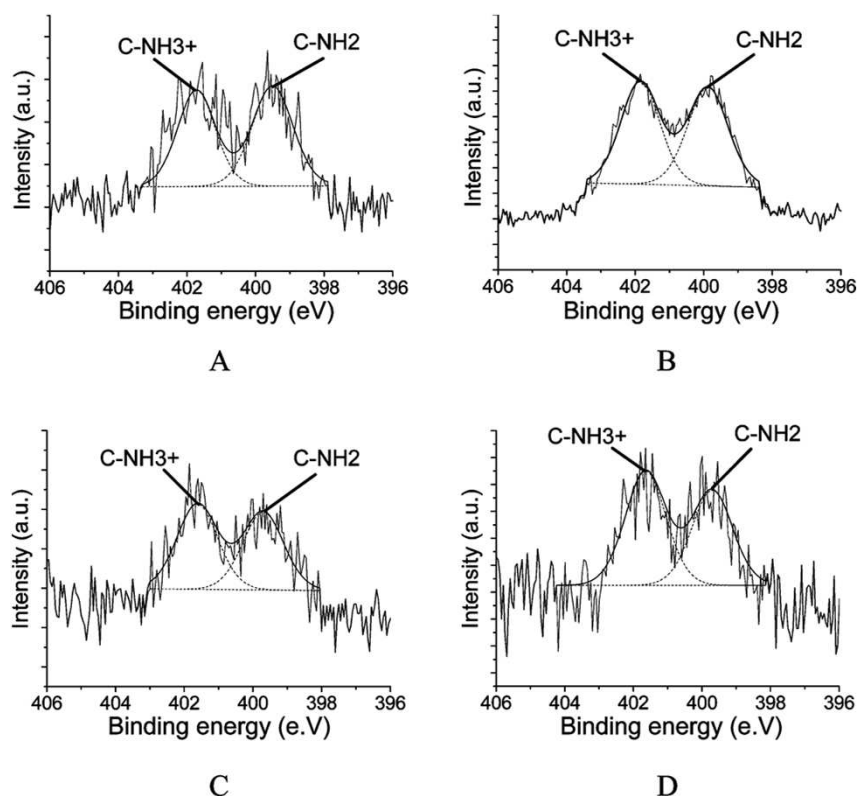
Figure 7. XPS analysis (N1s spectra) of amine FDU-12 samples synthesized with different amount of APTES: (A) APTES 15-160-1/20, (B) APTES 15-160-1/15, (C) APTES 15-160-1/10, and (D) APTES 15-160-1/7.5.
