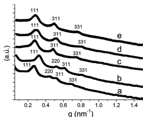
Figure 1. SAXS spectra of (a) FDU-12 PS synthesized at a reaction temperature of 15 °C and a hydrothermal temperature of 160 °C, and amine FDU-12 synthesized at different hydrothermal temperatures: (b) APTES 15-100-1/15, (c) APTES 15-130-1/15, (d) APTES 15-150-1/15, and (e) APTES 15-160-1/15.
