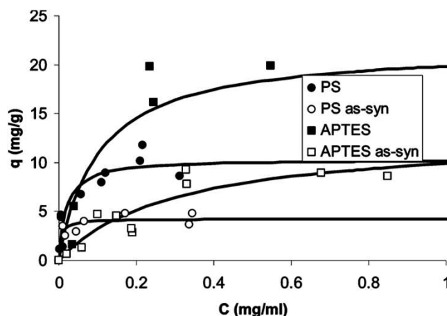
Figure 11. Adsorption isotherms of cellulase on PS, APTES 15-160-1/15, and their as-synthesized forms (at 4 °C).
