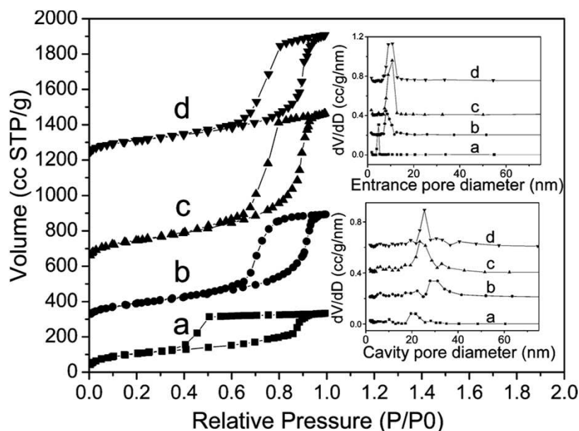
Figure 2. N_2 sorption isotherms of amine FDU-12 samples synthesized at different hydrothermal temperatures: (a) APTES 15-100-1/15, (b) APTES 15-130-1/15, (c) APTES 15-150-1/15, and (d) APTES 15-160-1/15 (inset: cavity pore size or entrance pore size distribution). The isotherm curves b, c, and d are shifted by 300, 600, and 1200 cc\ g^{-1}\ STP , respectively, for clarity.
