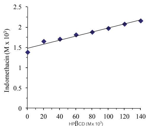
Figure 2. Phase solubility diagram of indomethacin in water containing various concentrations of HP \beta CD at 30 \pm 0.5°C ( n = 3 ).
