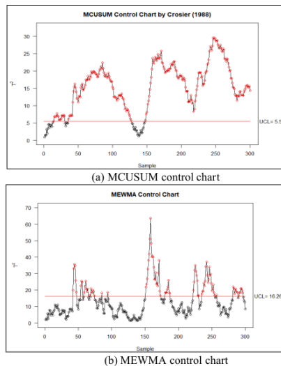
Figure 6. Multivariate control charts using residuals data
