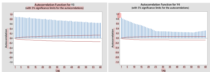
Figure 3. Autocorrelation test of each variable
