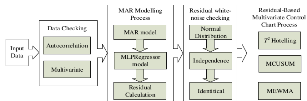
Figure 1. Procedure to build the proposed control chart
