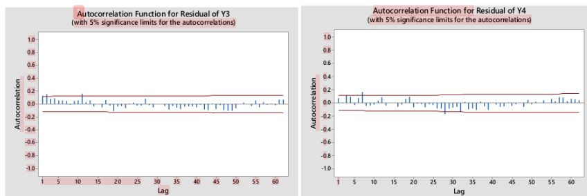
Figure 4. Autocorrelation test of each residual variable
