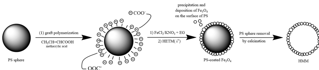
Fig. 1. The schematic mechanism of the HMM fabrication.
