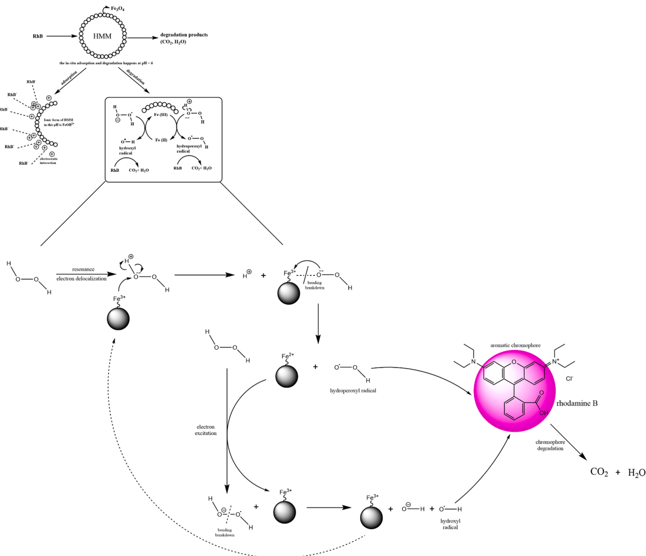
Fig. 11. The proposed mechanism of the simultaneous adsorption and degradation of \text{RhB} using HMM.
