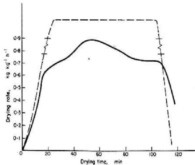
FIGURE 2. Drying rate
