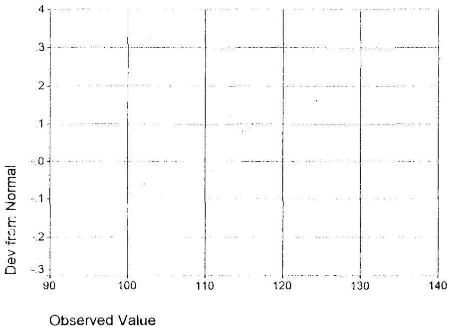
Detrended Normal Q-Q Plot of IM
