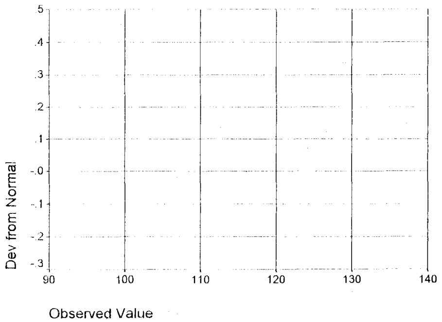
Detrended Normal Q-Q Plot of MHMDYH
