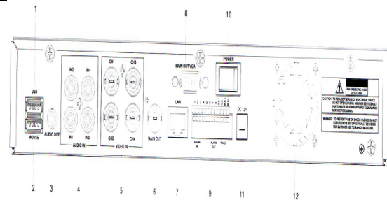
Gambar 8. Tampak belakang DVR
