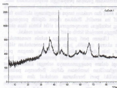
Gambar 2. Difraktogram Katalis Cu-Zn-Al/ \gamma - Al_2O_3
