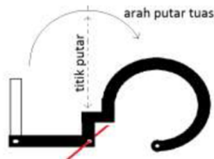
Gambar 9. Model tuas pendorong jari
