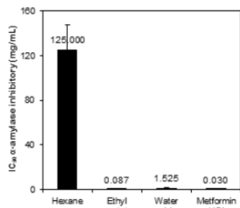
Figure 5. IC 50 values of starch digestion inhibition by \alpha -amylase compared to metformin hydrochloride as the reference drug.
