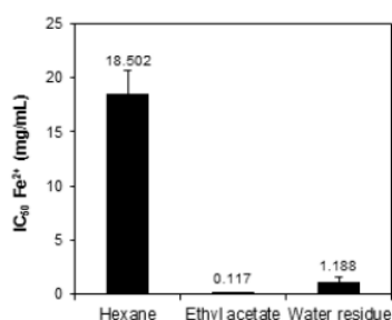
Figure 4. IC 50 values to the inhibition of Fe 2+ .
