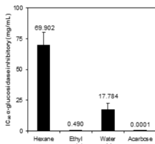
Figure 6. IC 50 values of starch digestion inhibition by \alpha -glucosidase compared to acarbose as the reference drug.
