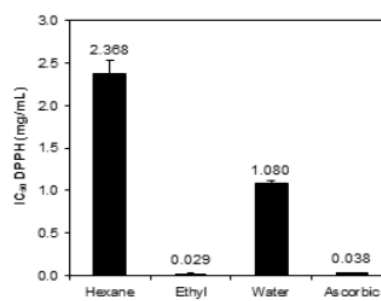
Figure 3. IC_{50} values to the inhibition of DPPH. Ascorbic acid was selected as positive control.
