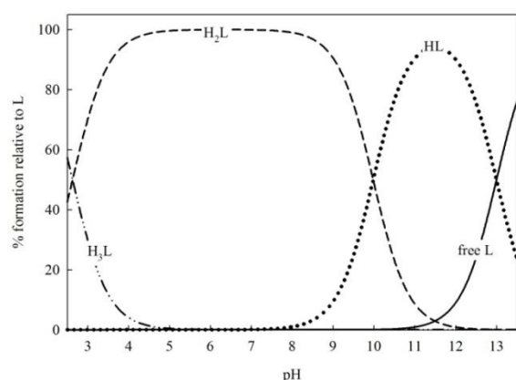
Figure 2. Species Distribution of 2,3-DHBA
