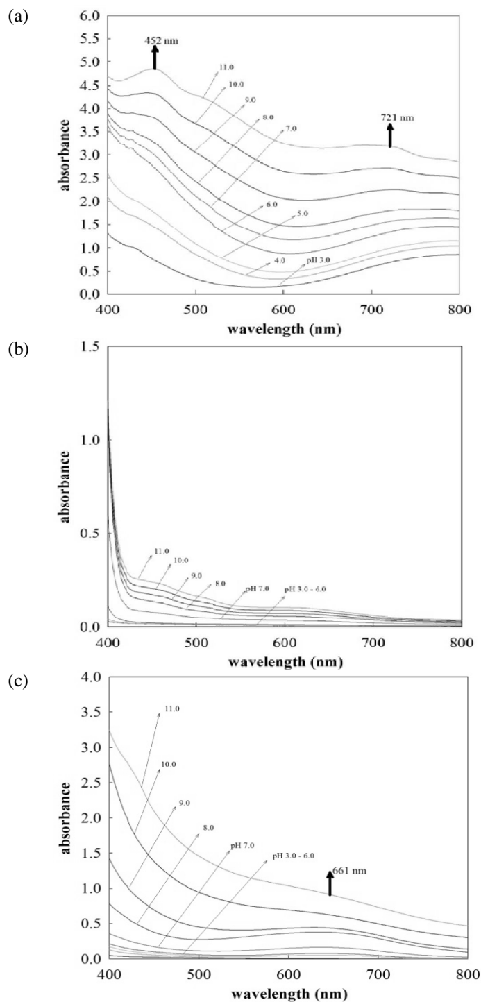
Figure 5. Spectrum of the (a) Copper, (b) Zinc and (c) Manganese system
