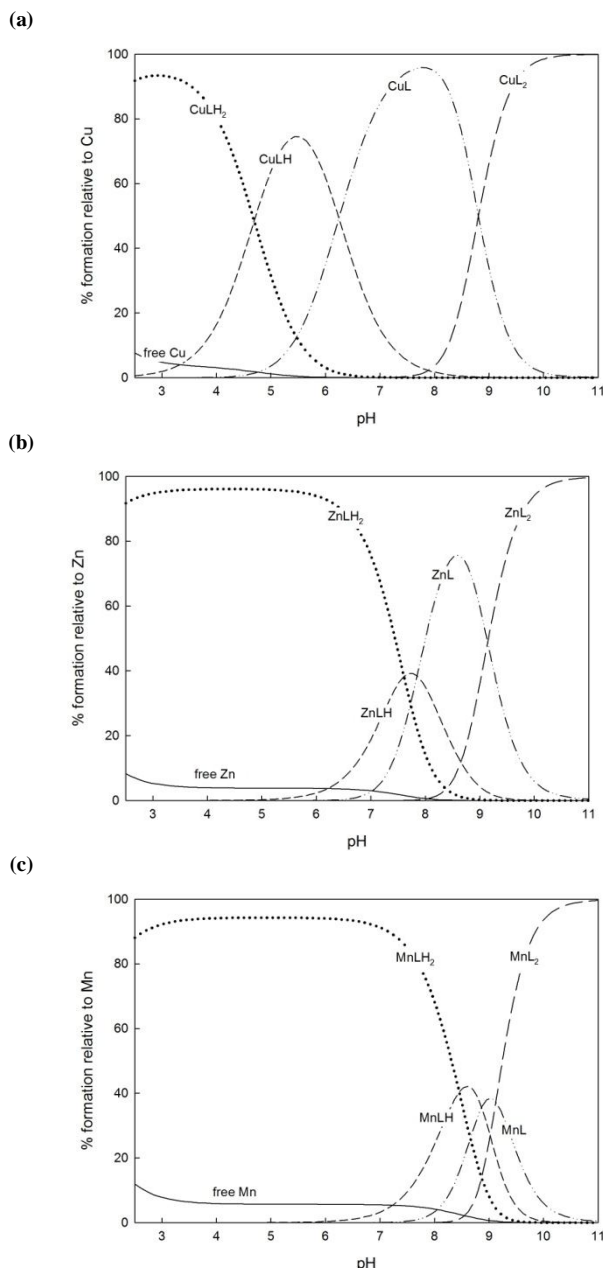
Figure 4. Species distribution of (a) Cobalt (b) Nickel and (c) Copper system
