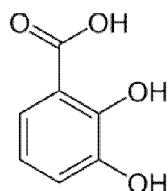
Figure 1. Structure of 2,3-dihydroxybenzoic acid
