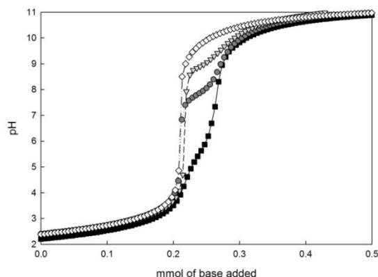
Figure 3. Titration curve of the system with metal to ligand ratio 1:2. \diamond , Ligand system; \triangle , \text{Cu}^{2+} -ligand system; \bullet , \text{Zn}^{2+} -ligand system; \blacksquare , \text{Mn}^{2+} -ligand system;
